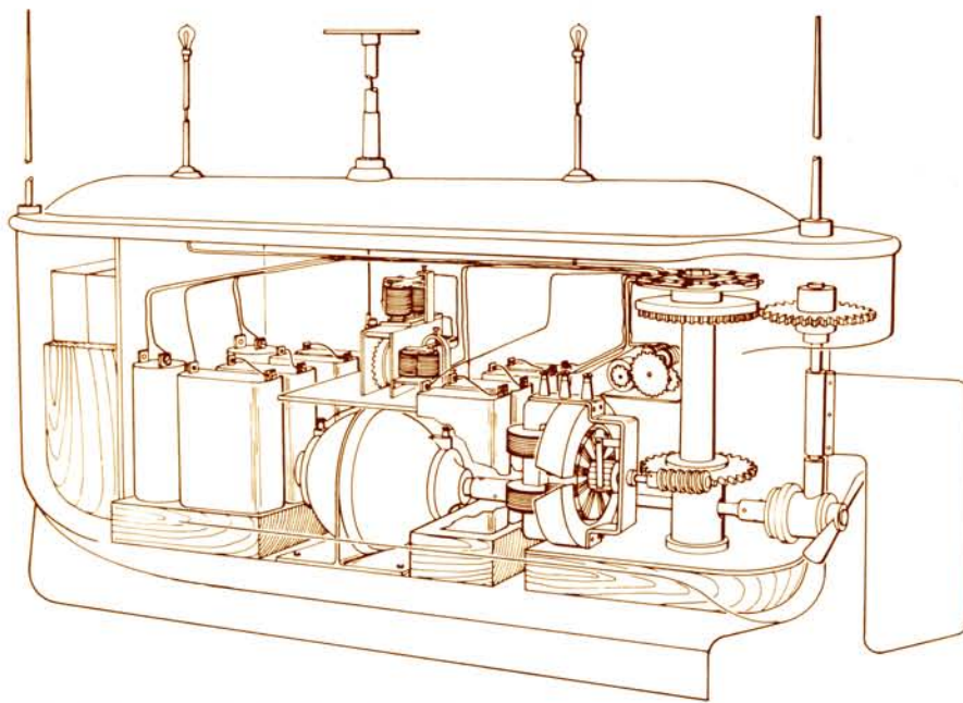
Above: Details of Tesla's amazing boat paralleled many of today's principles. Included in its radio system was a feed-back servo. He also developed a loop antenna. The proportional control servo and gear system to the rudder shows clearly, as does the electric drive motor, shaft and propeller. His location of batteries, relays, and equipment look very familiar across three-quarters of a century. Below: His RC submarine models were demonstrated to a perplexed Navy before the Spanish-American War. They could pump out water ballast.
